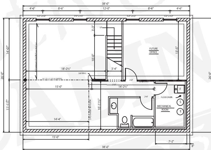
Foundation Plan
